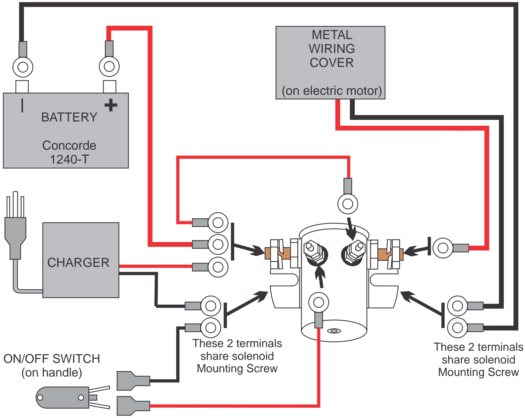
Model Thundervolt Wiring Diagram
